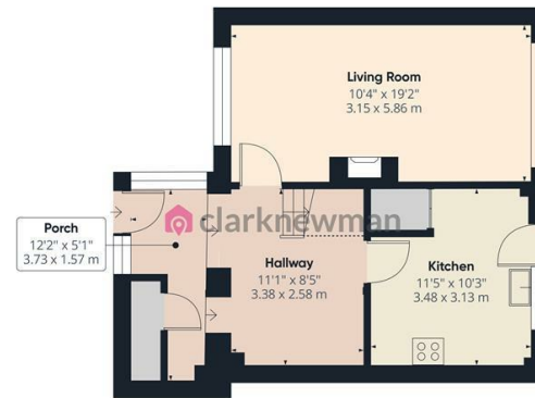
Floor 0 Building 1
